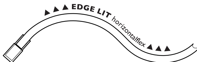
EDGE LIT illumination via side edge, horizontal bend. Standard length: 10m
